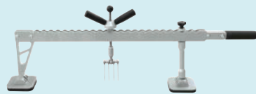
Double action levelling bar ref. 053564
